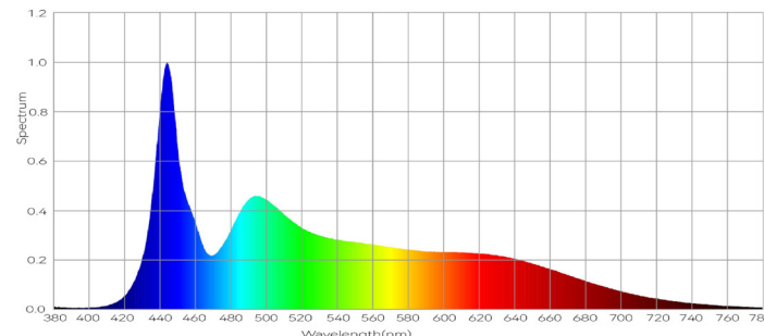
2835 BLUE DAYLIGHT COLOR SPECTRUM & WAVELENGTH CCT 10518K Ra=96.9
